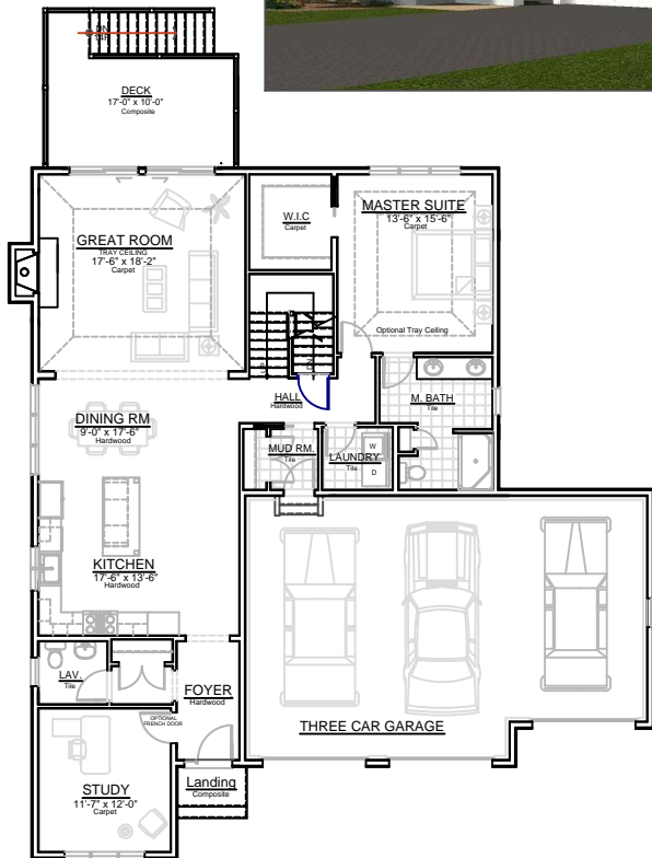
FIRST FLOOR PLAN Living Area: 1,684 S.F.
