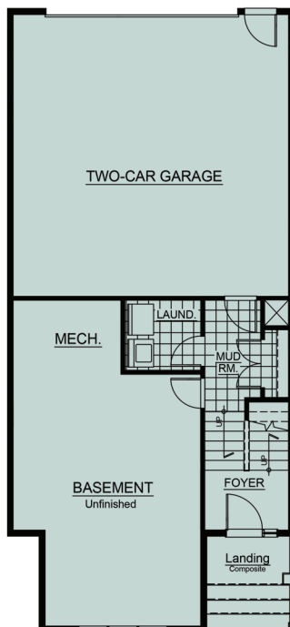
Lower Level | 120 SF
