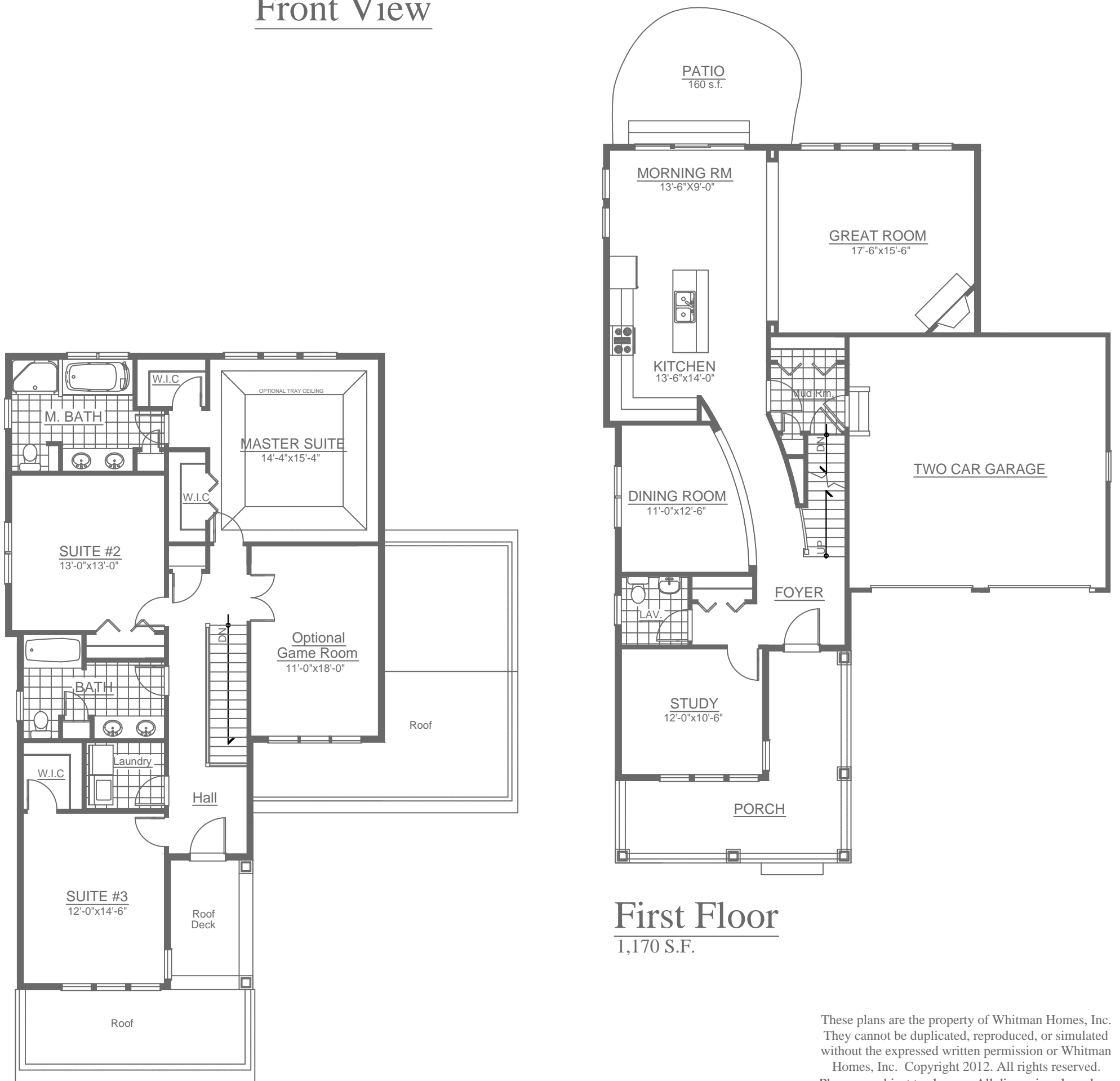
Second Floor 1,390 S.F.
