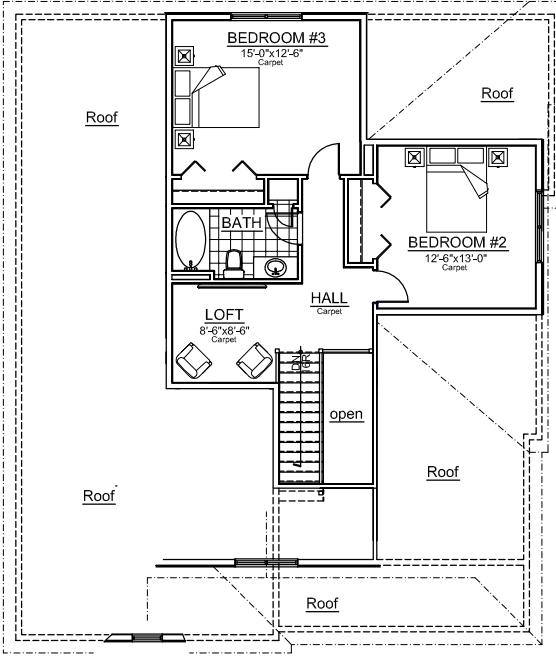
SECOND FLOOR PLAN LIVING AREA: 658 S.F.
