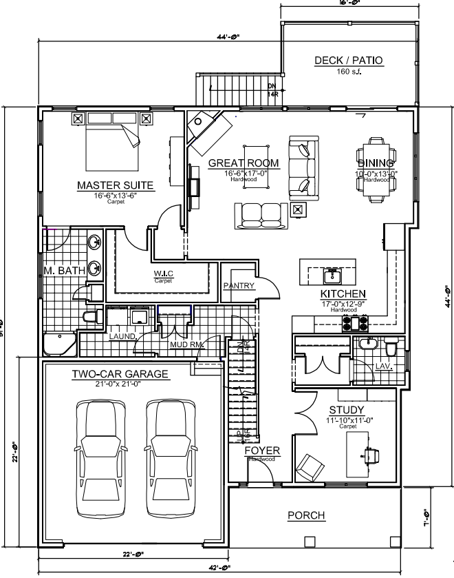
FIRST FLOOR PLAN LIVING AREA: 1,580 S.F.
