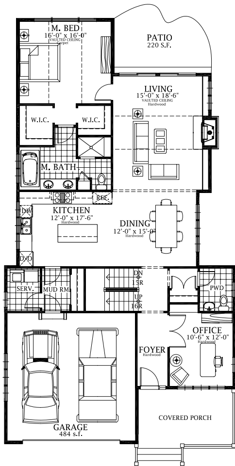
LOWER FLOOR 1,640 s.f.
