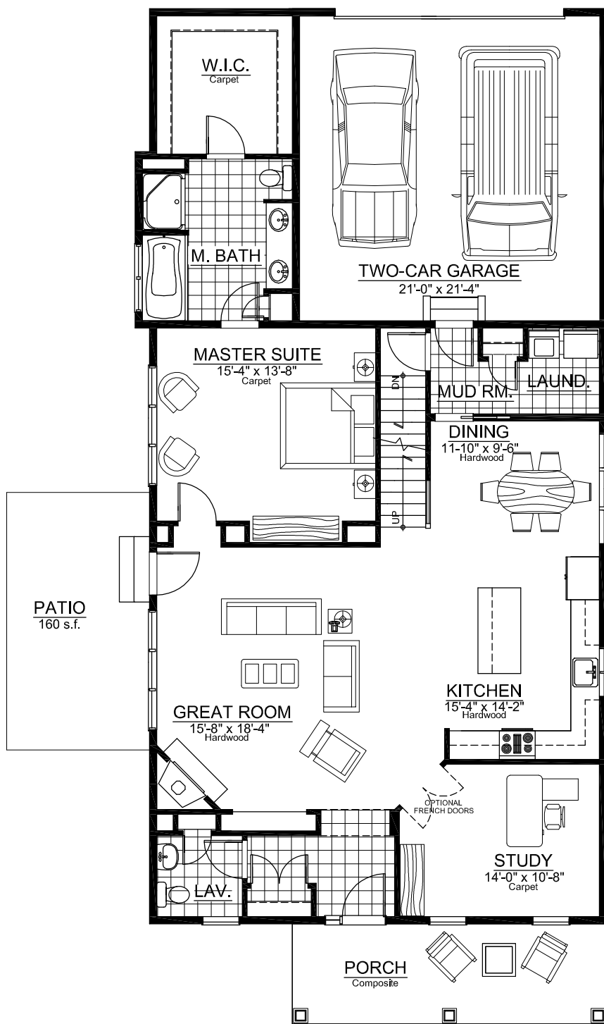
First Floor 1,588 S.F.
