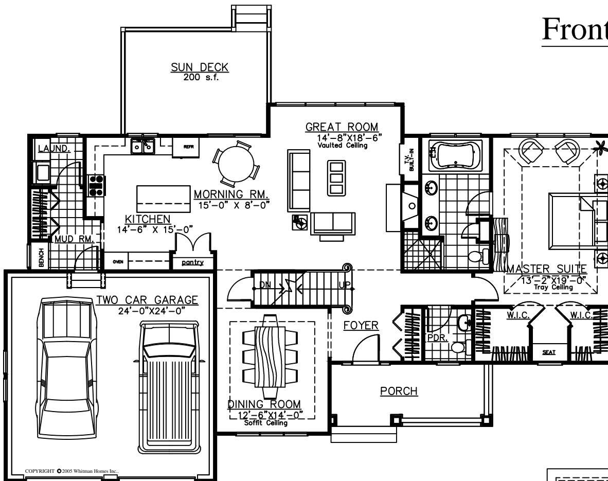
First Floor 1,660 S.F.
