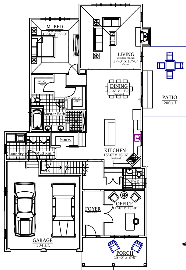
LOWER FLOOR 1,680 s.f.
