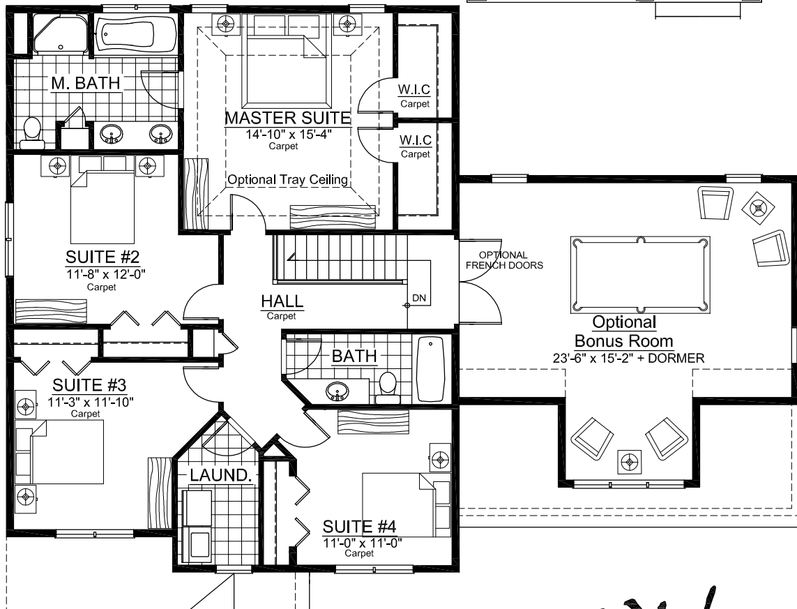
Second Floor 1,250 S.F.
