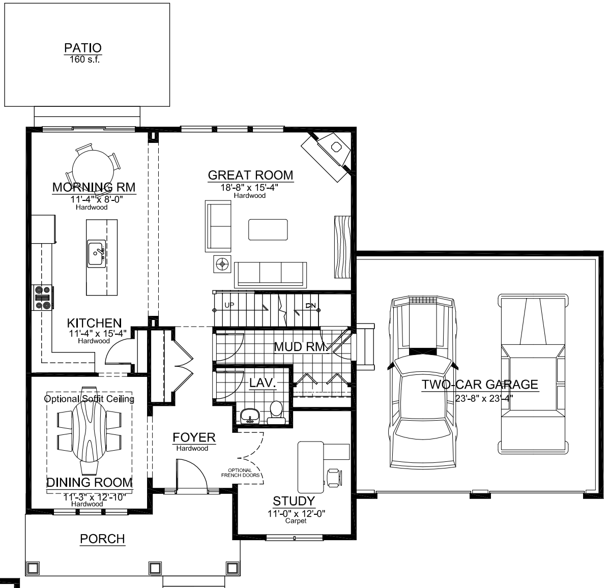
First Floor 1,215 S.F.
